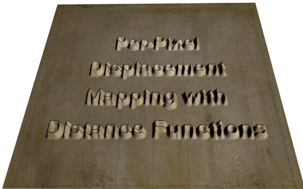
Figure 8-3. Rendering Displaced Text Because of the fine detail, text is a difficult case for some per-pixel displacement algorithms, particularly those based on uniformly spaced sampling. Note that our algorithm correctly captures occlusion between letters without aliasing.
